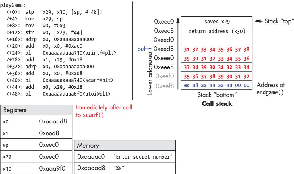
Figure 9-19: A sample string that can force secret to execute the endGame function
