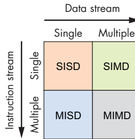
Figure 15-1: Flynn's taxonomy classifies the ways in which a processor applies instructions.
