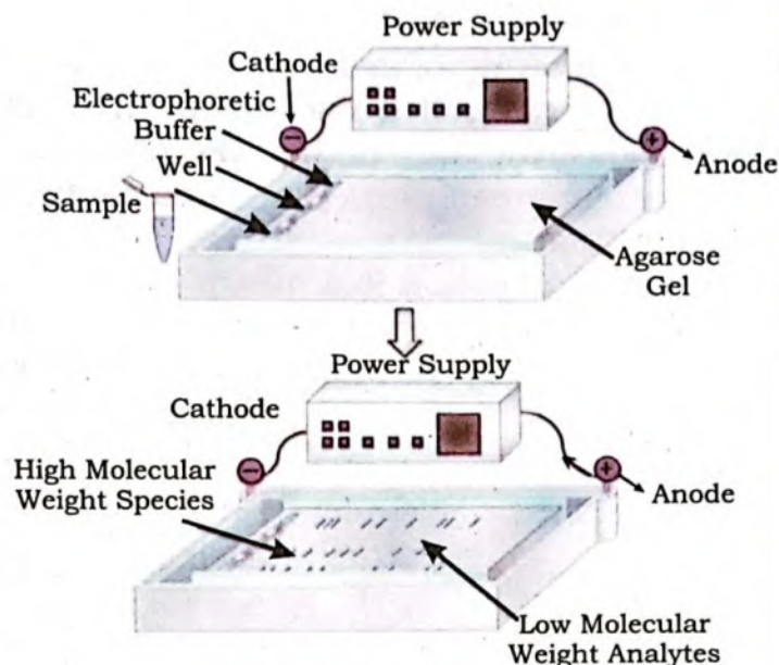
Fig 3.5 Electrophoresis
