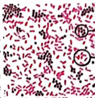
Fig 3.2 Differential staining
