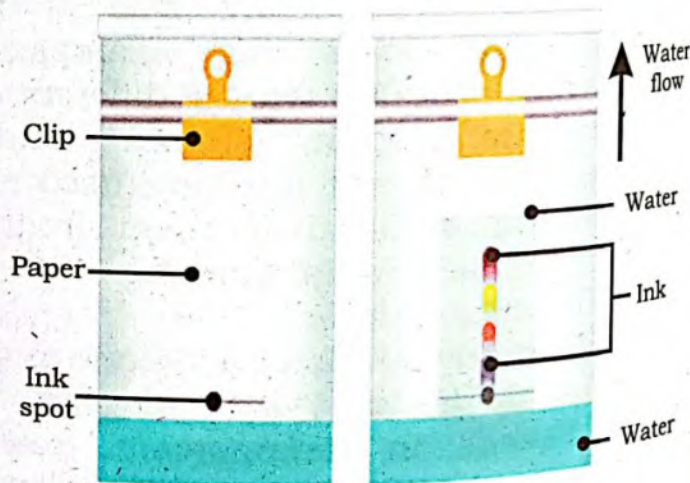
Fig 3.4 Paper chromatography
