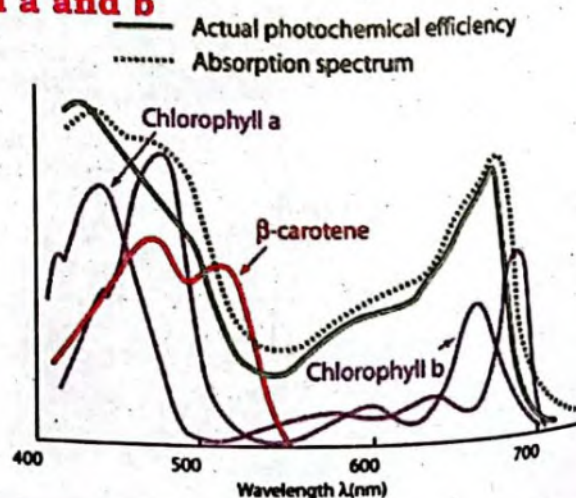
Fig 4.4 Absorption graph
