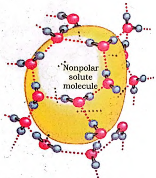
Fig 1.5 Vaporization
