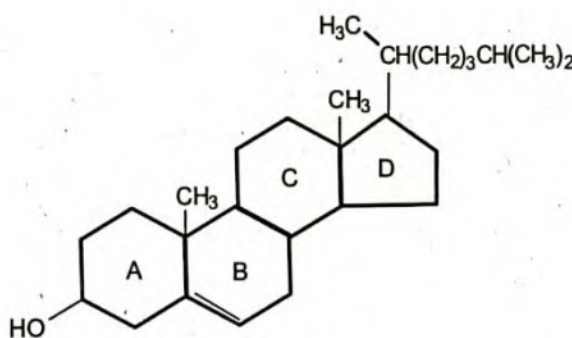
(b) Cholesterol
