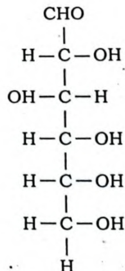
Glucose
