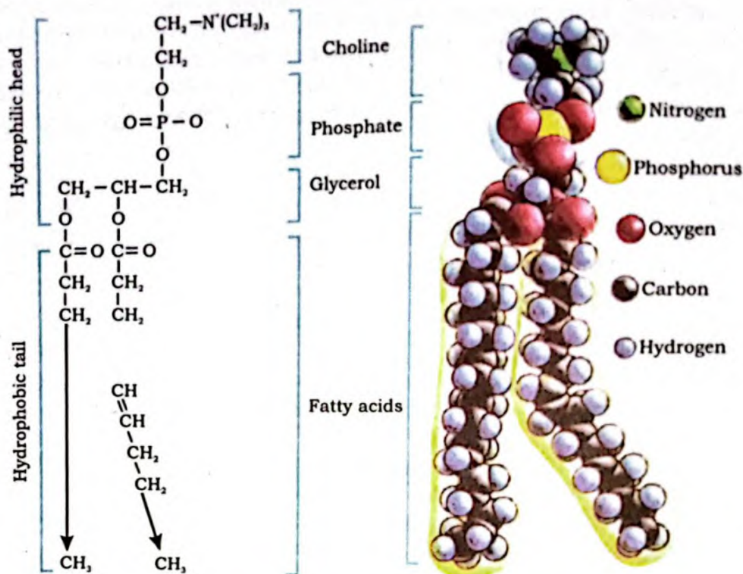
Fig 1.12 Phospholipid
