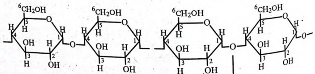
Amylopectin
