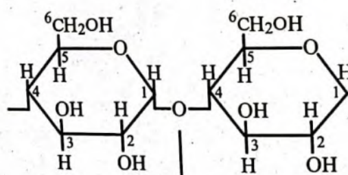
α1-4 glycosidic linkage
