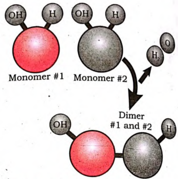
Fig 1.1 Condensation reaction
