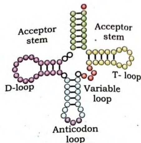
Fig 1.16 tRNA
