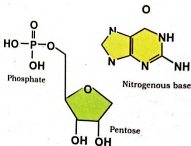
Structure of nucleotide
