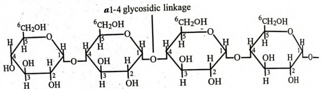
Amylose
