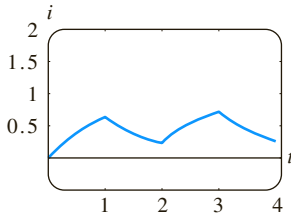
FIGURE 7.4.5 Graph of current i(t) in Example 9
