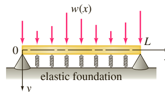
FIGURE 7.R.11 Beam on elastic foundation in Problem 48
