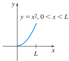
FIGURE 11.3.10 Function f in Example 3 is neither odd nor even.
