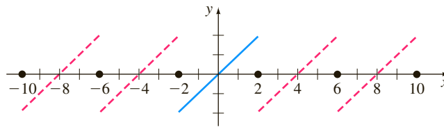
FIGURE 11.3.4 Periodic extension of function shown in Figure 11.3.3
