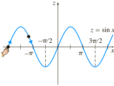
FIGURE 10.4.4 -\pi/2 and 3\pi/2 are stable in Example 2
