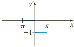
FIGURE 11.2.2 Piecewise-continuous derivative f' in Example 2
