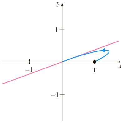
(a) degenerate stable node
