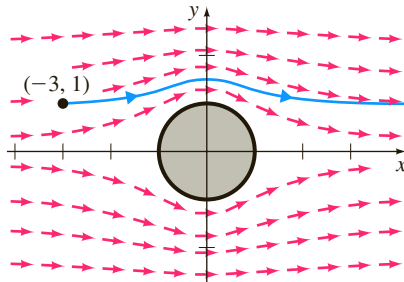
FIGURE 10.1.1 Vector field of a fluid flow in Example 3
