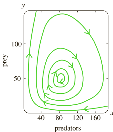
FIGURE 10.4.10 Phase portrait of the Lotka-Volterra model in Example 3
