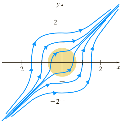
FIGURE 10.3.8 Phase portrait of nonlinear system in Example 8
