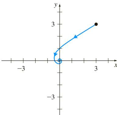
FIGURE 10.1.5 Solution curve in Example 6
