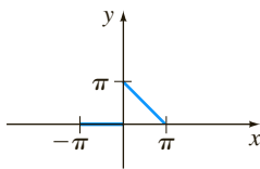
FIGURE 11.2.1 Piecewise-continuous function f in Example 1
