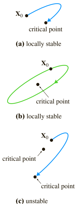
FIGURE 10.2.1 Critical points
