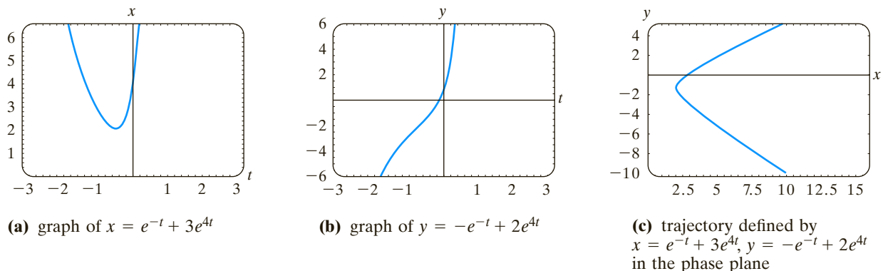
FIGURE 8.2.1 A solution from (5) yields three different curves in three different planes
