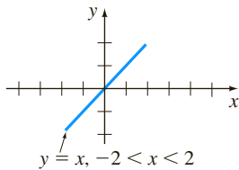
FIGURE 11.3.3 Odd function in Example 1
