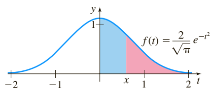
FIGURE 14.1.1 Bell curve
