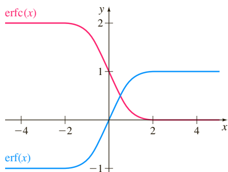
FIGURE 14.1.2 Graphs of \operatorname{erf}(x) and \operatorname{erfc}(x)
