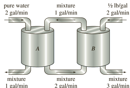
FIGURE 8.3.1 Mixing tanks in Problem 11
