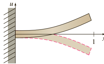
FIGURE 12.7.4 Vibrating cantilever beam in Problem 11
