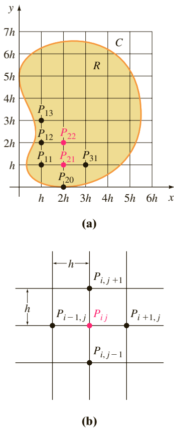
FIGURE 15.1.2 Region R overlaid with rectangular grid
