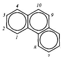
Phenanthrene
