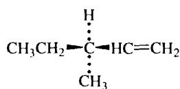
( S )-3-Methyl-1-pentene
